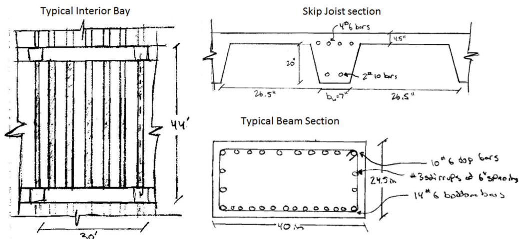
Figure 5 - 1: One way joist and beam system details
