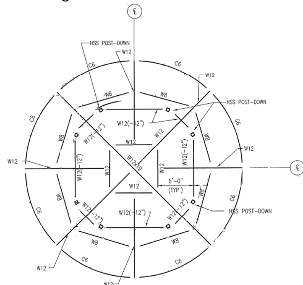
Figure 2-8: Turret roof framing plan
